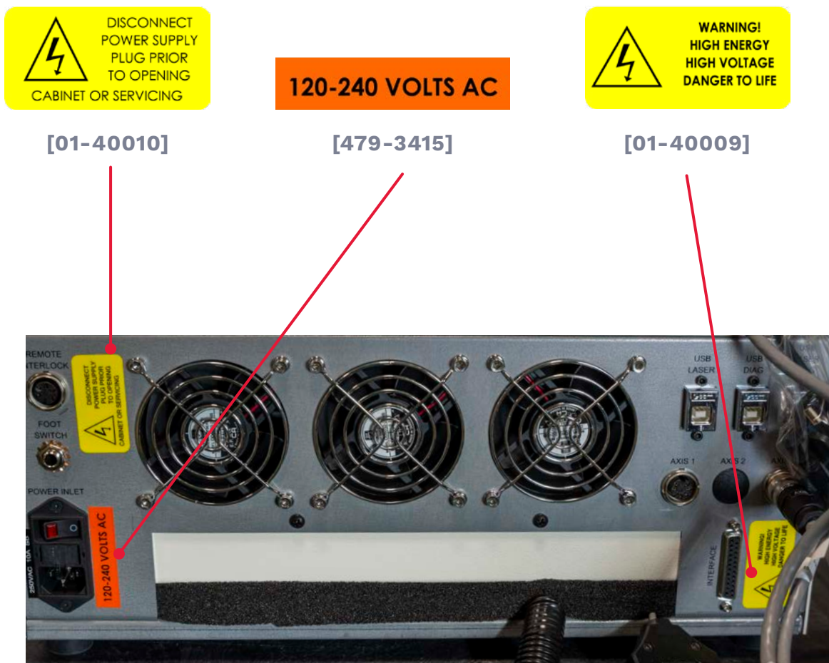
Figure 5 (3802 Series rear view)
