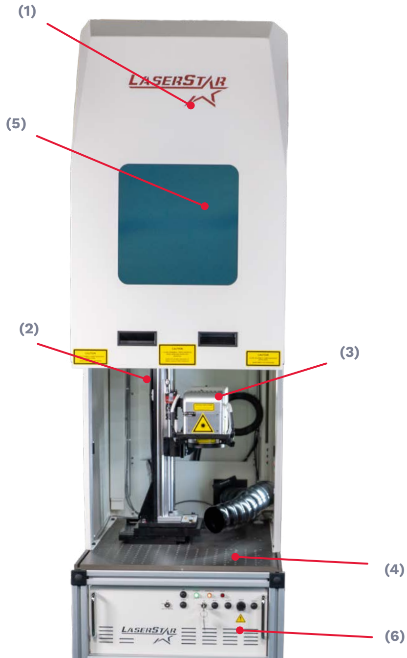
Figure 1 (FiberCube® 3802 Series Marker)
