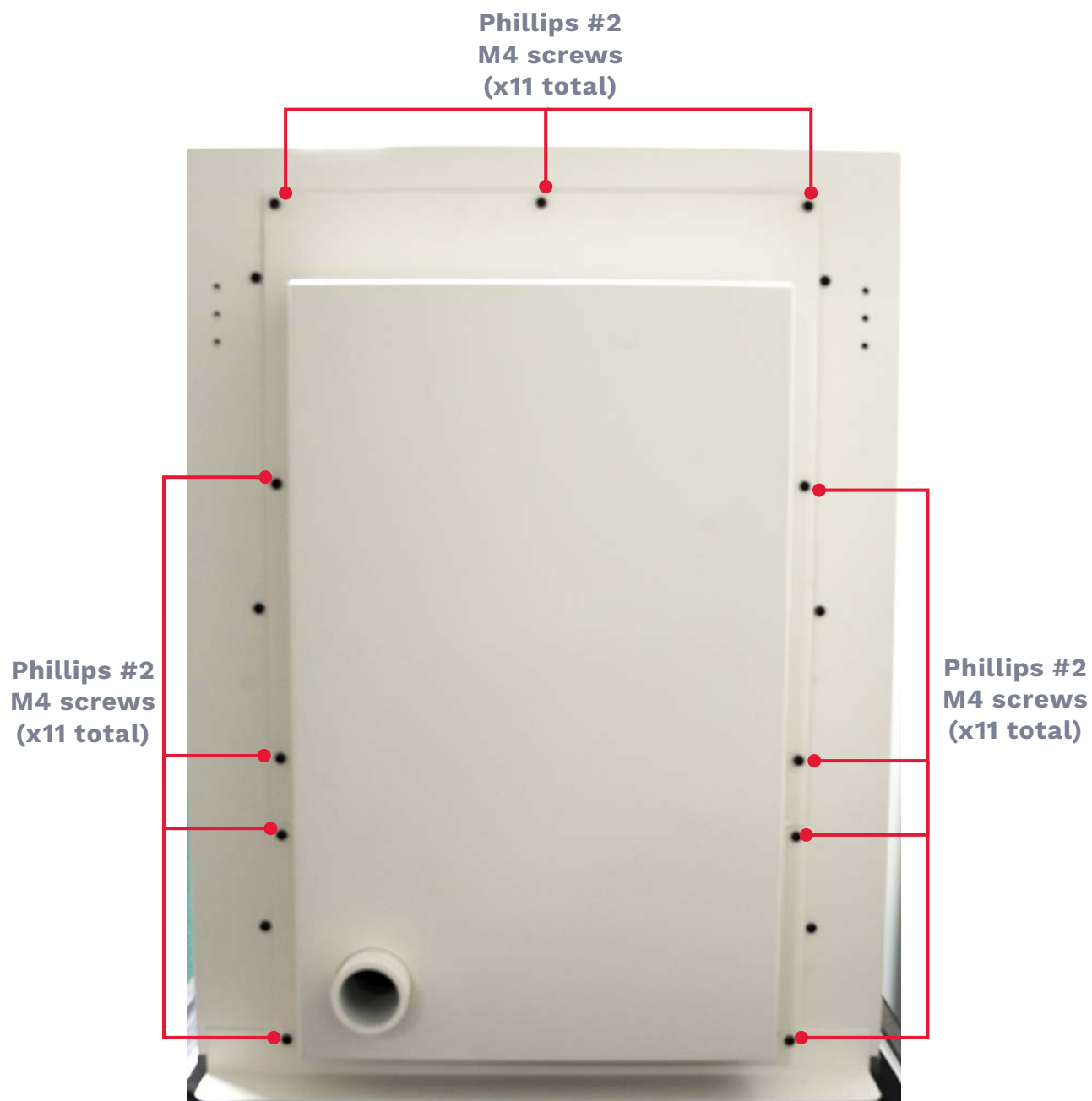
Figure 9 (3802 Series rear view)
