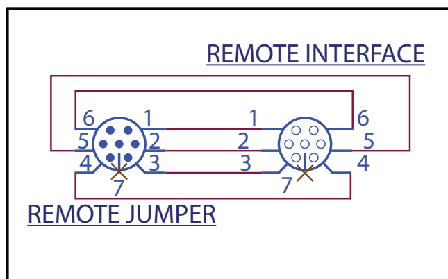
Remote Interlock Shorting Connector / Plug PN-185-30-5009
